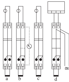
Simple current transformer test circuit: a= Normal operation b= Measured value testing c= Transformer testing d= Relay testing
