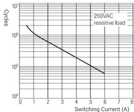
Electrical endurance-Resistive load
